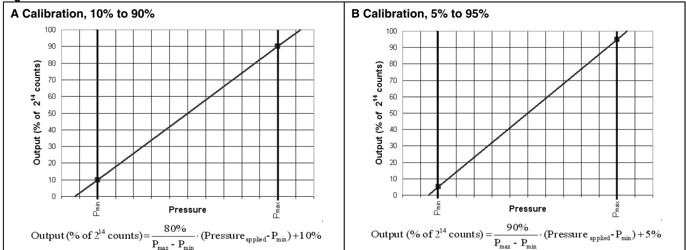
Figure 2. Transfer Functions and Limits
